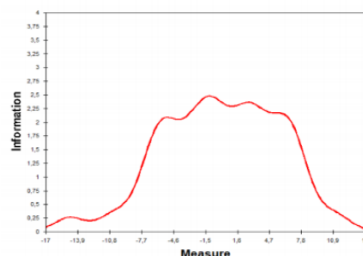
Figure 1. Test Information Function
