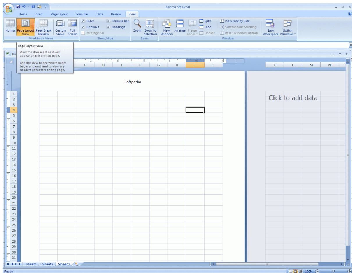
OFFICE 2007 Screenshot
