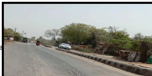
Figure 21 Shoulder width is not provided, full length fences are not provided and huge area under land acquisition reducing road width
