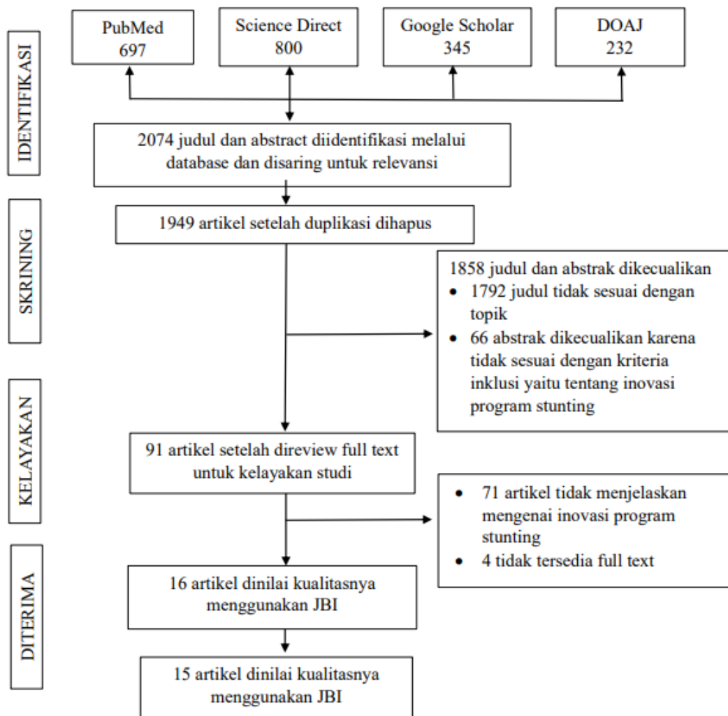
Figure 1. PRISMA Flowchart
