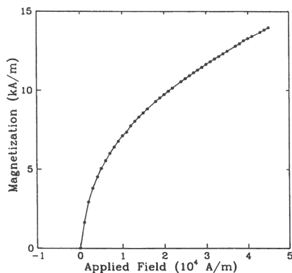
Fig. 1. Magnetization as a function of applied field. (Note that "Fig." is abbreviated and there is a period after the figure number followed by two spaces.) (Cambria 10pt)
