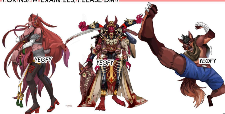
CELLSHADE EXAMPLE
