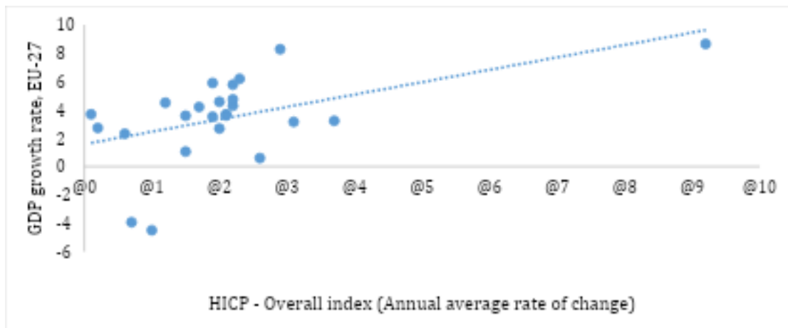
Figure 2. A linear model of the relationship between the overall HICP and GDP growth in the EU-27
