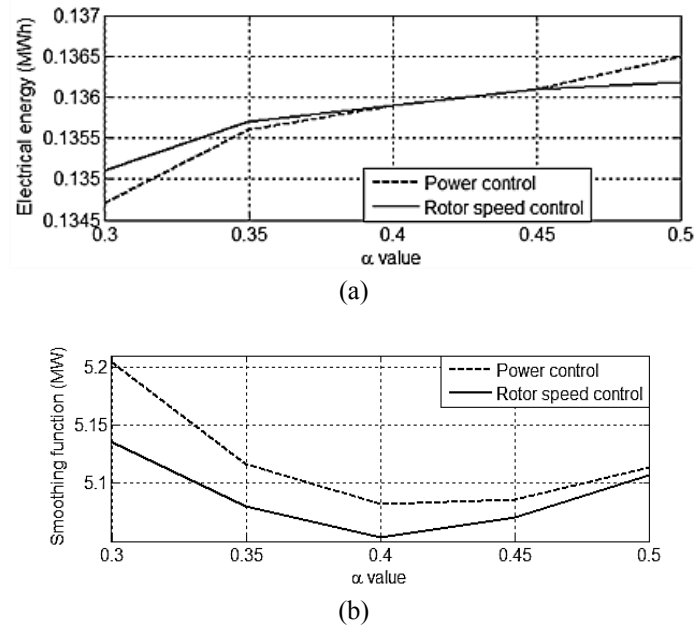
Figure 2. Comparing simulation results in wind turbine performance with the power control mode to that with the rotor speed control mode in (a) energy output and (b) smoothing function
