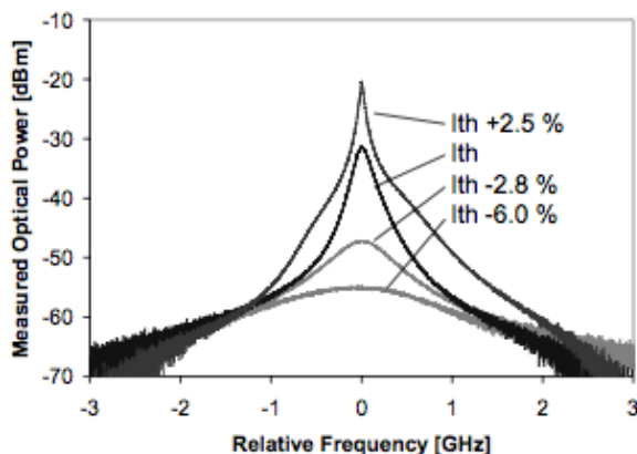
Fig. 1. Spectral shape evolution of the DFB with increasing bias current. Wavelength has been shifted to center for all measurements.
