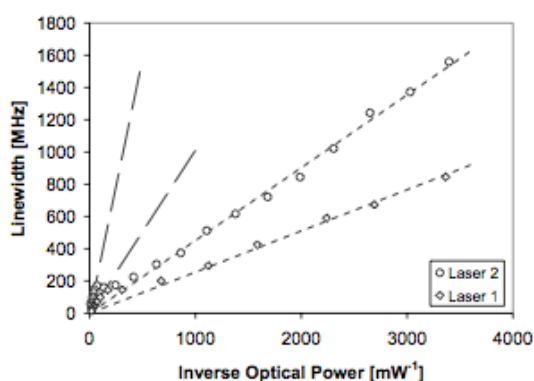
Fig. 4. Linewidth versus inverse power around the threshold region for both lasers. Long dashed lines stand for the Henry asymptotic behaviour (2) and short dashed lines for the Schawles-Townes asymptotic behaviour (1)
