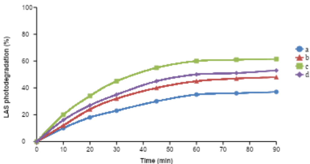
Fig 5. Effect of the reaction time on the LAS photodegradation over \text{TiO}_2\text{-Cr(200)-Cu(2)} with various masses, as (a) 10 mg, (b) 20 mg, (c) 30 mg, and (d) 50 mg
