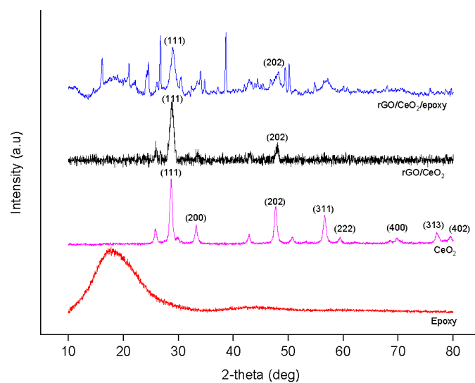
Fig 3. Diffractogram pattern of epoxy, \text{CeO}_2 , rGO/ \text{CeO}_2 , and rGO/ \text{CeO}_2 /epoxy composite
