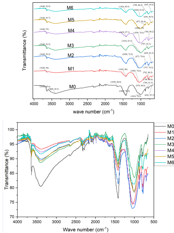
Figure 10. FTIR spectra of the M0, M1, M2, M3, M4, M5 and M6 mixes after 28 days of curing
