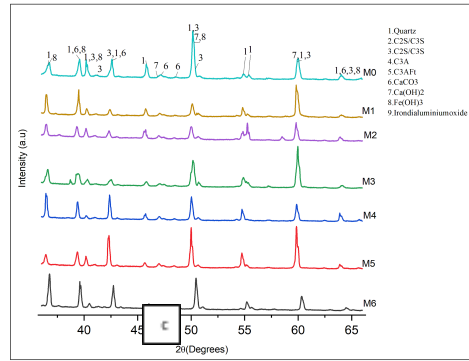
Figure 8c. XRD patterns of mortar mixes 65 ° -100°
