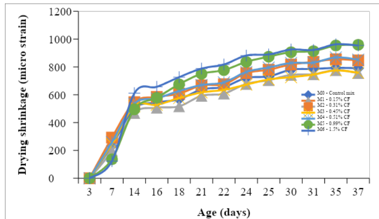
Figure 5. Drying shrinkage results of mortar mixes
