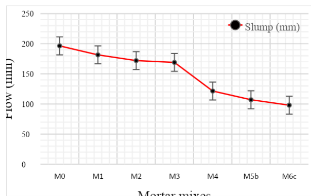
Figure 2. Flow curve of mortar mixes
