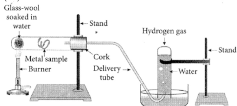
Action of steam on metal
