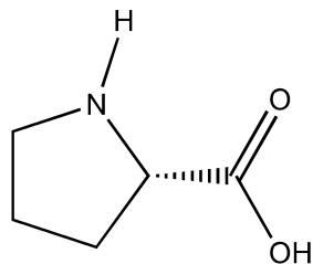
(S)-proline
