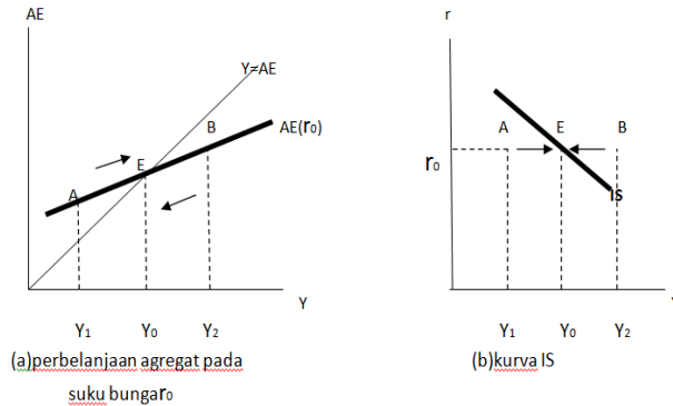
Gambar 1. Kurva IS
