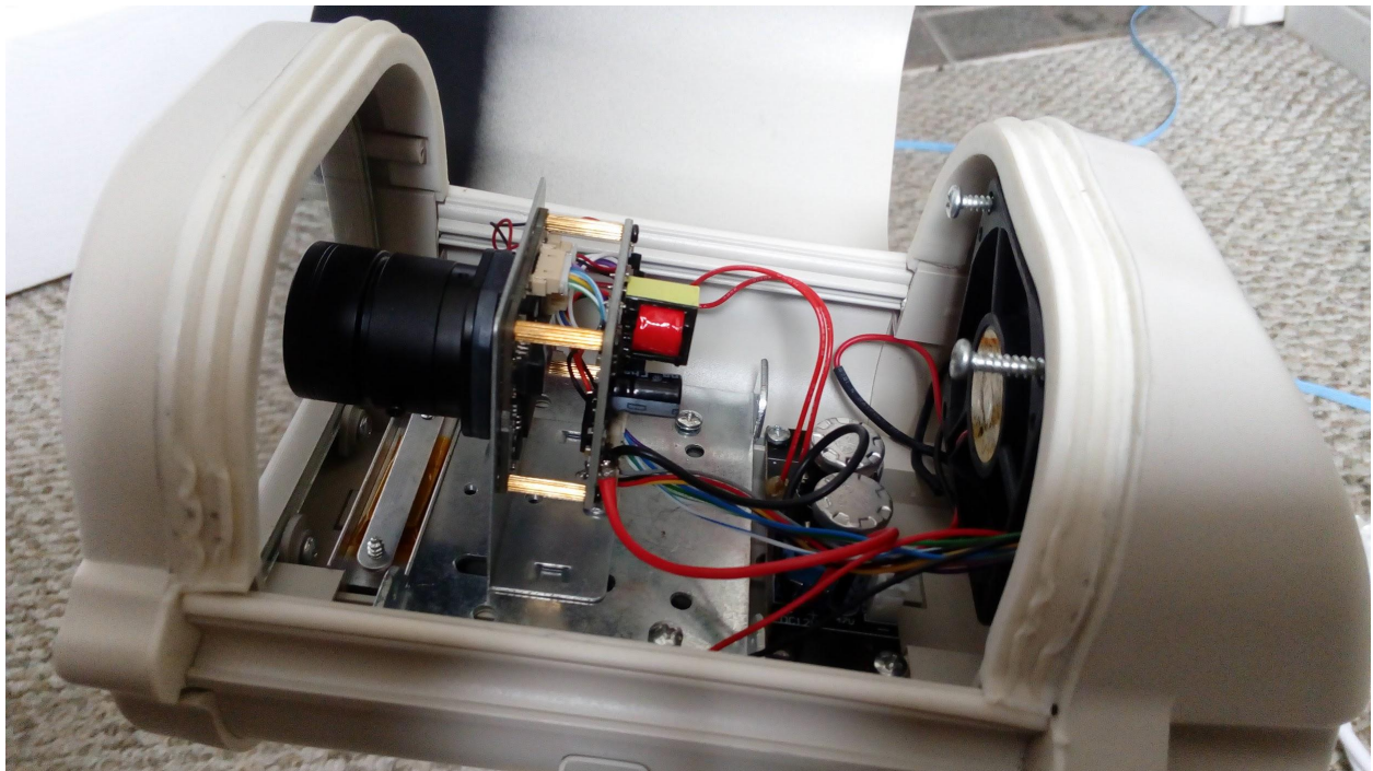
Completed camera with the 4mm lens
