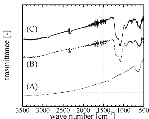
Fig. 1 FT-IR spectra of particles.
