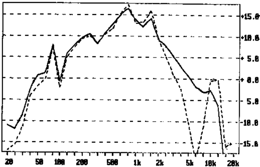
Figure 10: Two uncorrected right transfer functions of the same ear. Solid line with the probe against the eardrum, dashed with the probe pulled away, but still well within the ear canal.
