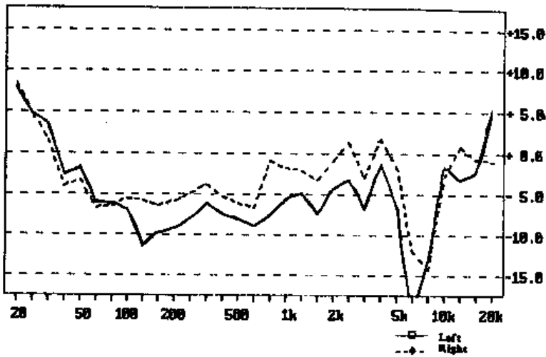
Figure 12. Correction curves for AKG 240 headphones on MC
