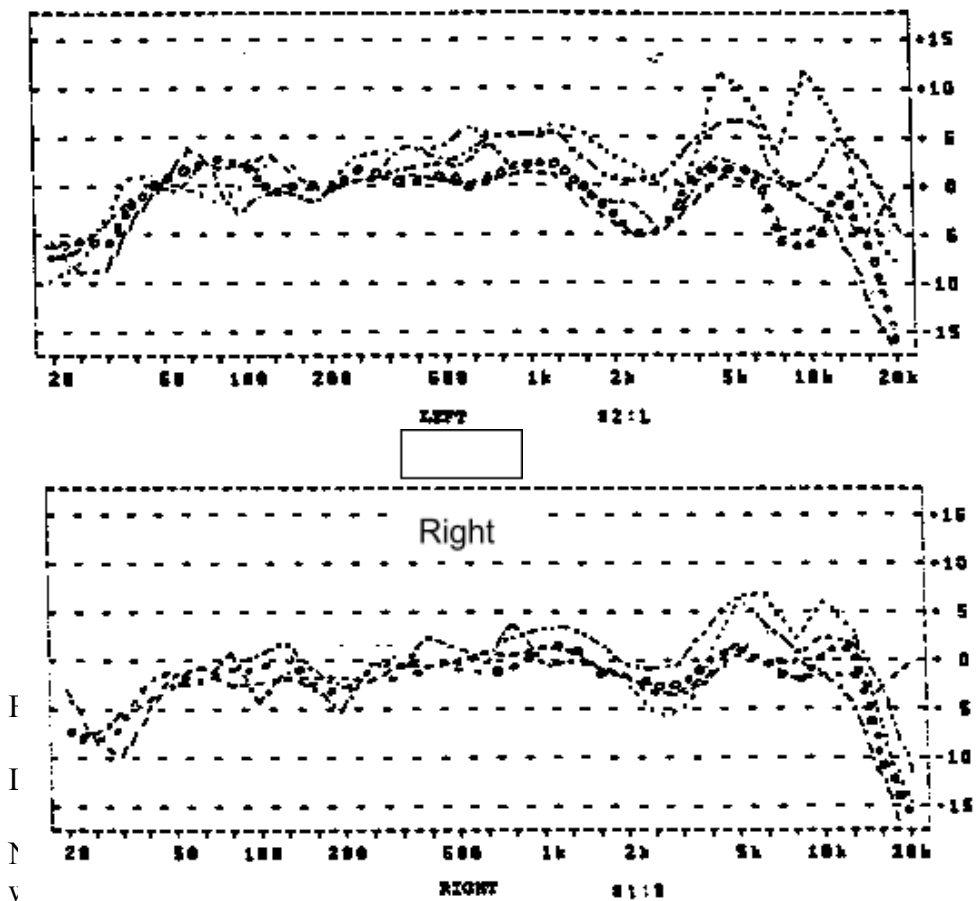
Response of KU-8li: - - - music A/B; ○○○○ 0° free field; ●●●● 30° free field; - · - · 90° free field.
