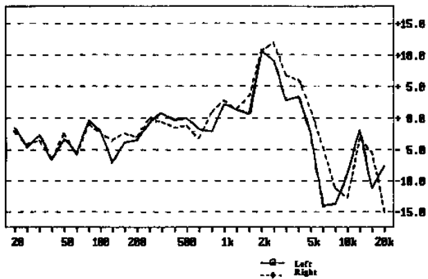
Figure 3. Forward Pinnae Response, PM
