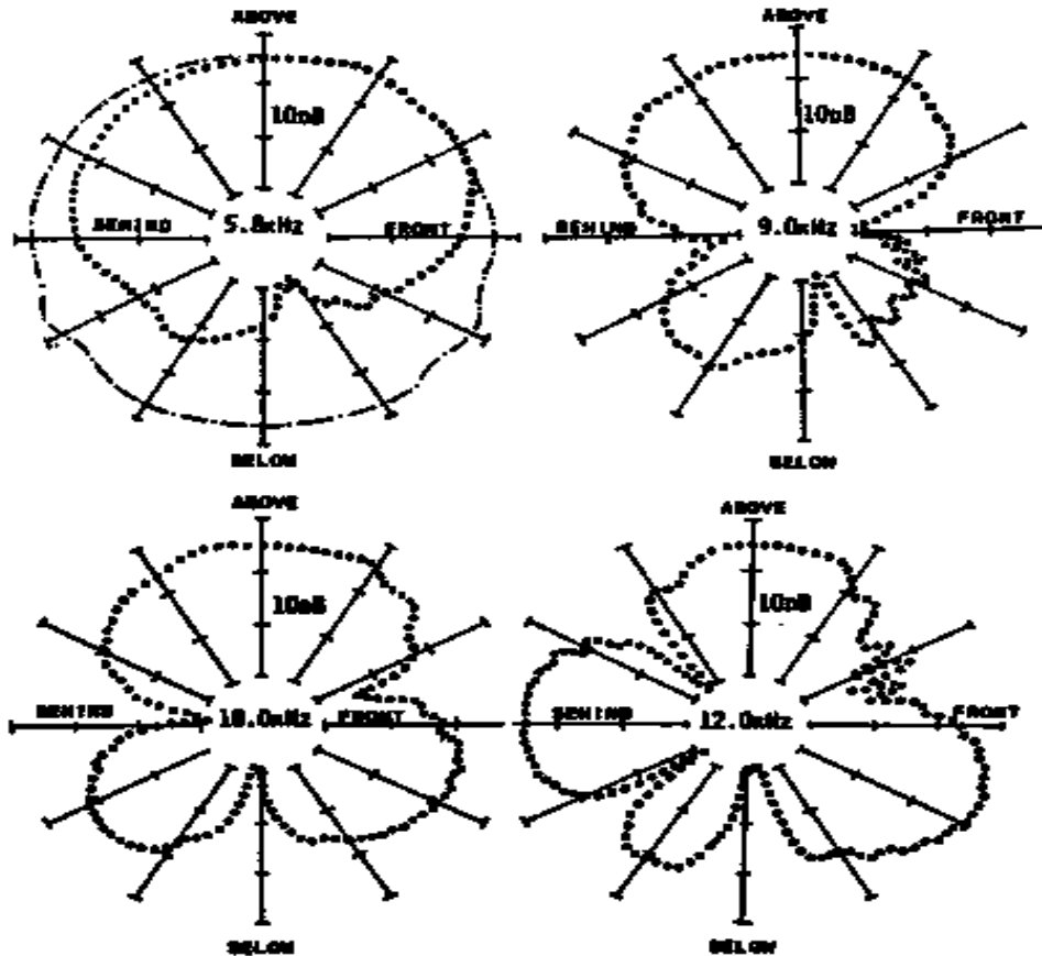
Figure 4. Vertical median plane directivity measured at a coupler microphone of KEMAR (without torso). Male adult pinna. " - . - " shows the directivity of the head alone at 5.8 kHz; pinna replaced by a flat plate. —From Kuhn
