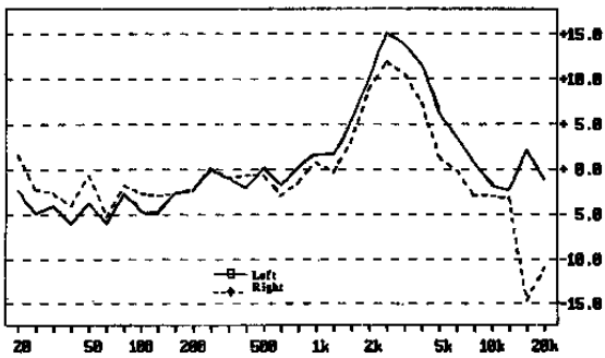
Figure 1. Forward Pinnae Response, DG
