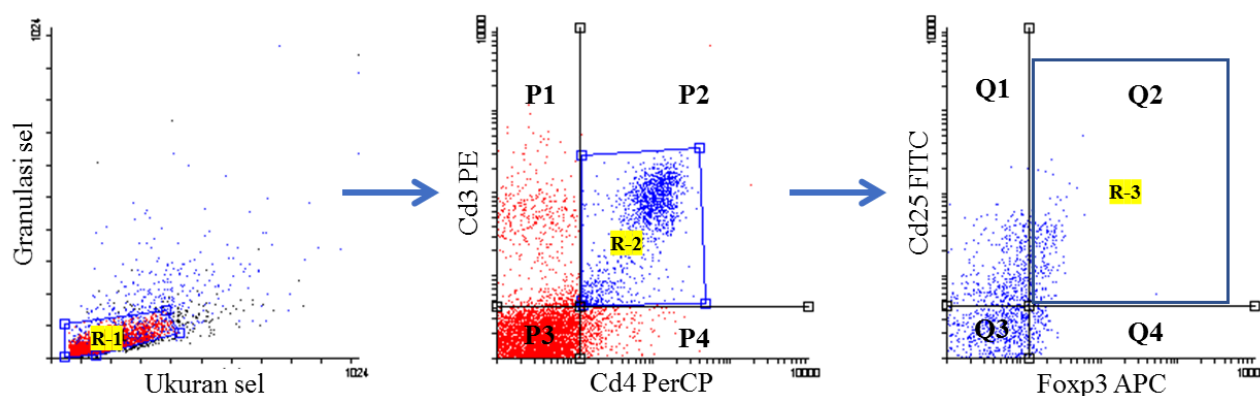
Gambar 1. Strategi gating
