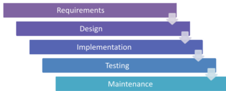
Gambar 1. Metodologi Waterfall
