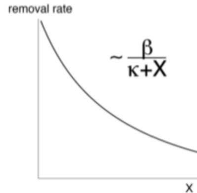
Figure 7.10: Removal rate per senescent cell drops with senescent cell abundance X.
