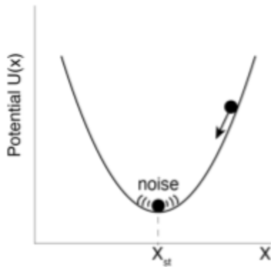
Figure 7.12: Damage dynamics can be likened to a particle in a bowl-shaped potential well jiggled by noise.
