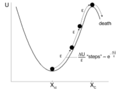
Figure 7.17: Death requires kicks in the same direction whose chance is exponentially small.
