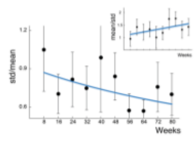
Figure 7.7: Coefficient of variation, defined as CV = \text{std}/\text{mean} , of senescent cells drops with age. Inset: 1/CV rises with age.
