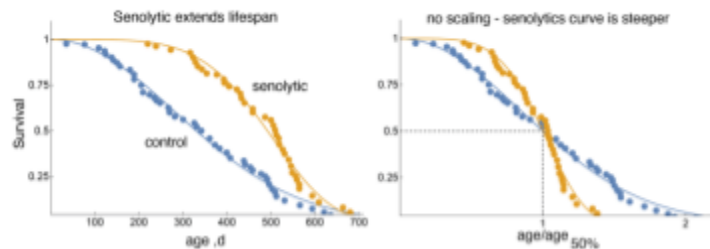
Figure 7.25: Senolytic drugs increase mean mice lifespan and show steepened survival curves as predicted by model. Adapted from (Kowald and Kirkwood 2021).
