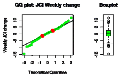
Figure 1. Data Distribution Compared Against Theoretical Normal Distribution
