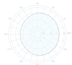
Typical horizontal pattern Omnidirectional 2S dipole
