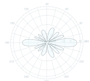
Typical vertical pattern 4-stack
