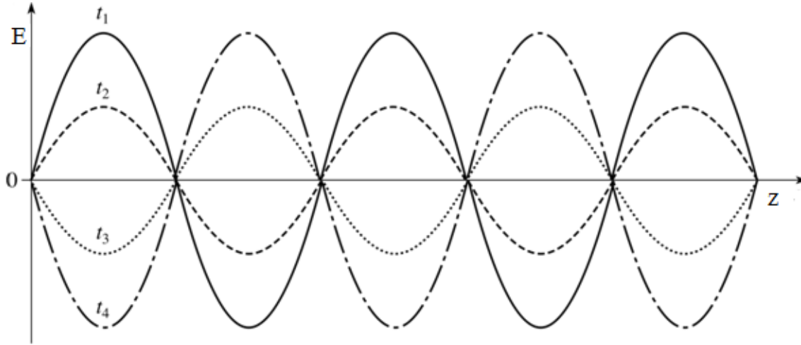
Figure 2, Illustrate the standing wave of \mathbf{E} = \text{Re}(\mathbf{e} \exp(i\omega t)) for different times t_1, t_2, t_3 .
