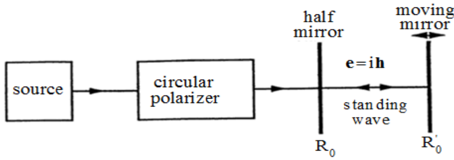
Figure 1. Schematic for the generation of parallel electromagnetic fields using two counter-propagating, orthogonally polarized light.
