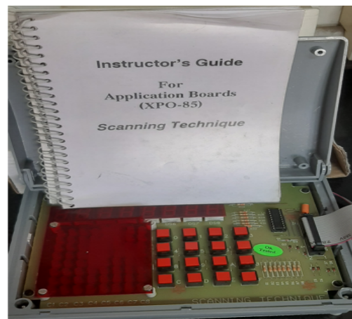
Analog to Digital Interfacing Card
