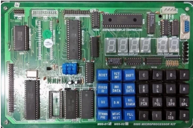
Microprocessor Trainer Kit 8085,
