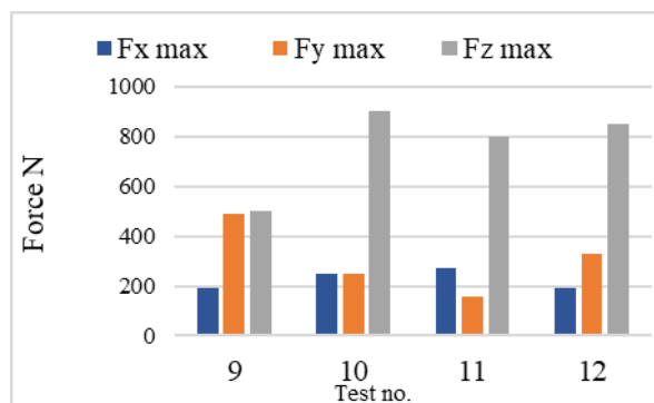
Fig. 1. Maximum forming force during various experimental runs
