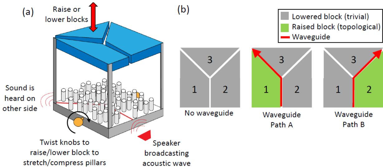
Figure 3: Exhibit of topological acoustic switch. (a) Three-section acoustic metamaterial system with compressible rubber pillars in an air-tight box. (b) By stretching or compressing the pillars to change the topological phases of the lattice segments, the system can block sound, or transmit sound along Path A or Path B.
