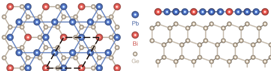
Figure 1: \text{Pb}_3\text{Bi} crystal structure on germanium \text{Ge}(111) [1].
