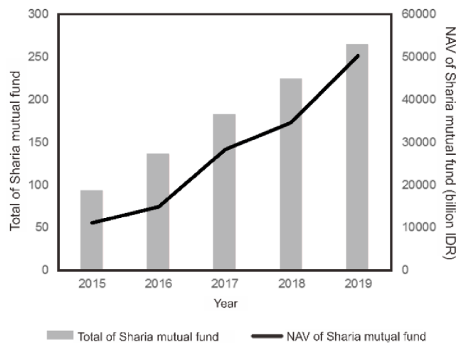
Figure 1. Growth in Sharia Mutual Funds Amount and NAV in Indonesia
