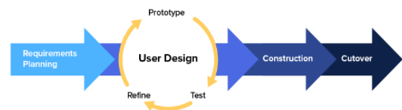
Gambar 1. Model RAD
