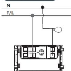
Interruptor Simples
