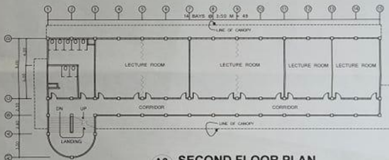
A2 SECOND FLOOR PLAN 02 03 SCALE 1 : 400 M
