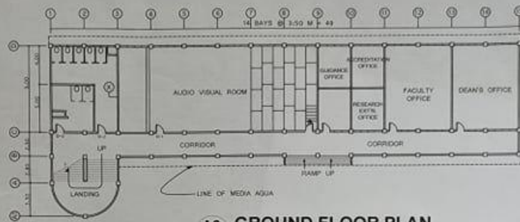
A2 GROUND FLOOR PLAN 01 03 SCALE 1 : 400 M
