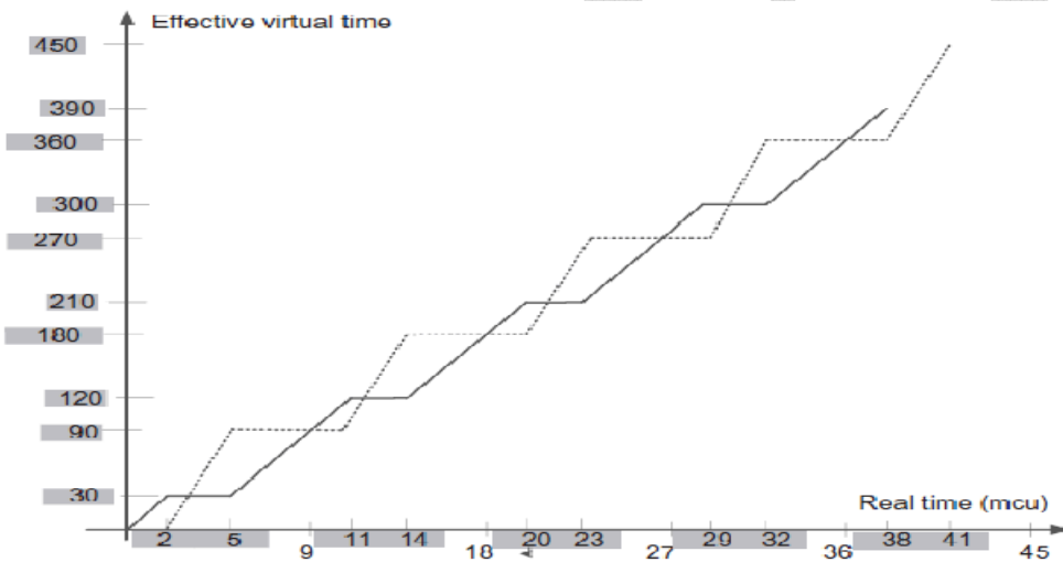
Figure 6.11 displays the effective virtual time and the real time of threads a and b . When a thread is running, its effective virtual time increases as the real time increases; a running thread appears as a diagonal line. When a thread is runnable but not running, its effective virtual time is constant. A runnable period is displayed as a horizontal line. We see that the two threads are allocated equal amounts of virtual time, but thread a , with a larger weight, consumes its real time more slowly.
