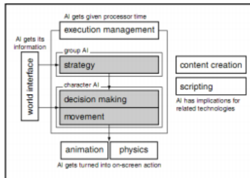
Gambar 1. Model game AI [1]
