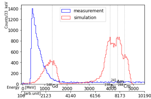
Figure 1. Example of an image output from alpha spectrometer
