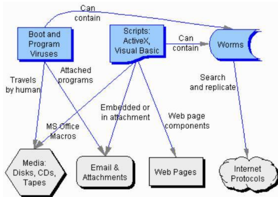
A simple diagram to show how malware can propagate
