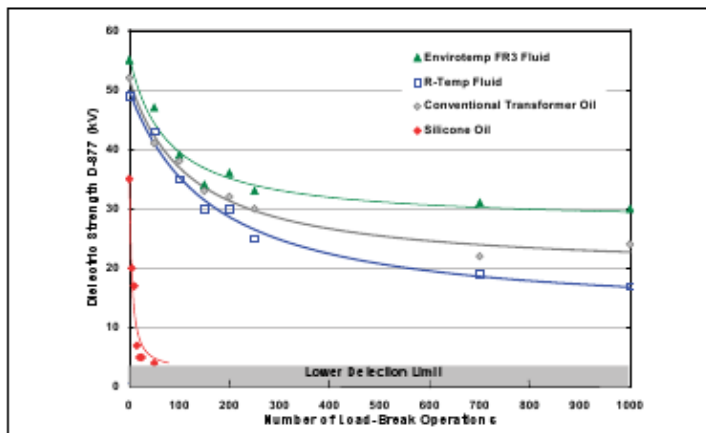
Figure 5. Fluid loadbreak dielectric strength retention comparison.
