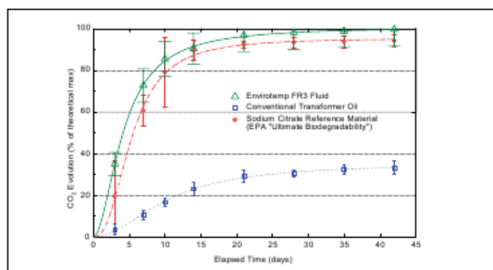
Figure 1. Aerobic Aquatic Biodegradation Graph EPA Test OPPTS 835.3100
