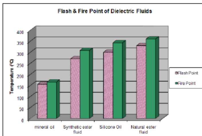
Figure 2. Flash & Fire Point of Dielectric Fluids (°C).
