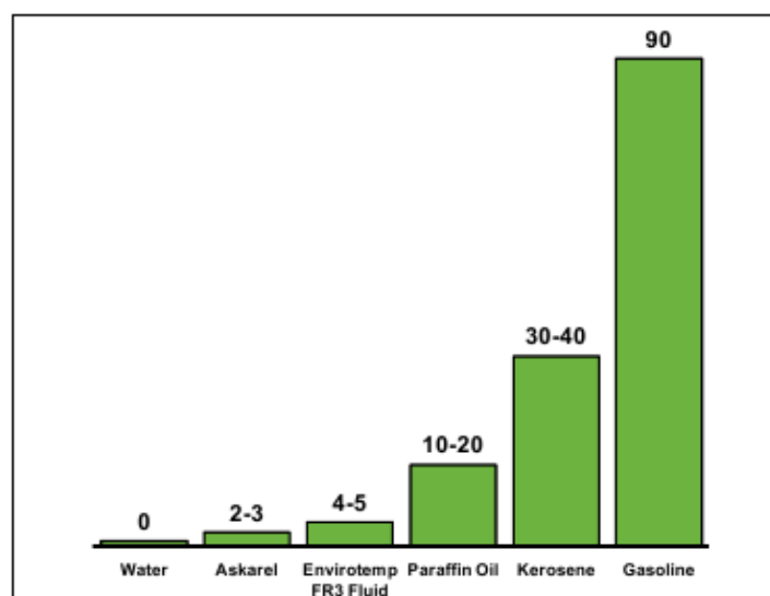
Figure 3. Fire Hazard Rating UL Standard 340.
