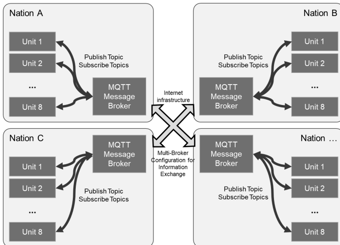
Figure 5 - Message-Broker setup in a multi-nation context. Adapted from (Johnsen, Manso and Jansen, 2020)
