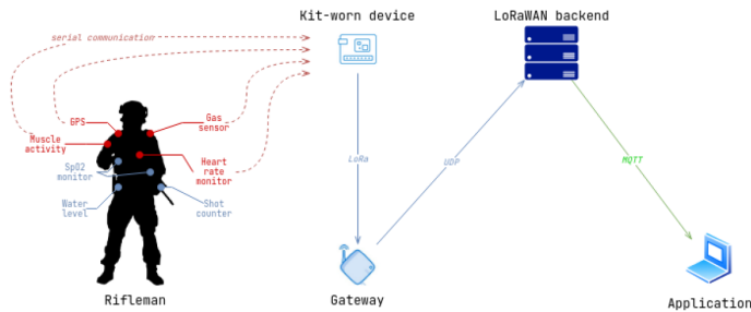
Figure 2: Soldier wearable high-level architecture
