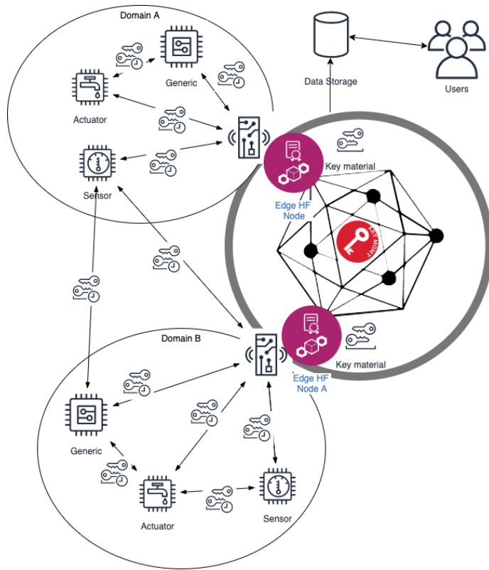
Figure 4 Distributed ledger-based key management and authentication for federated IoT environments.
