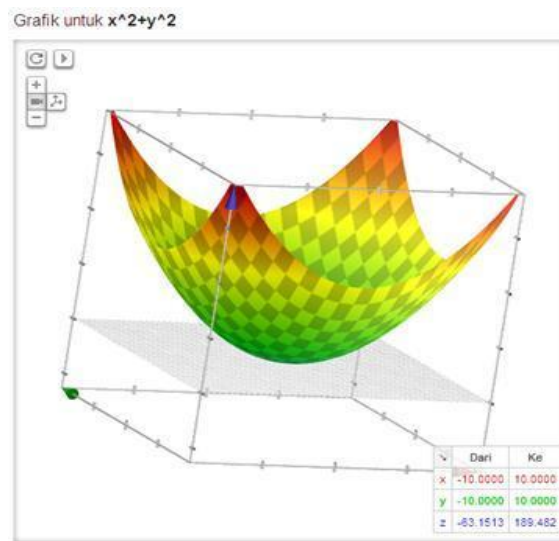
Figure 1. Graph Quadratic Equation
