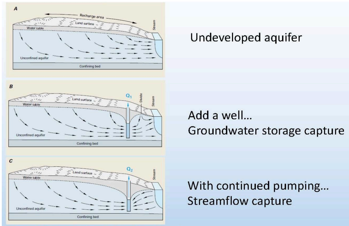
Figure 11. A cross-section of the development of a cone of depression (from OWRD presentation to Oregon Water Resources Commission December 3, 2021)
