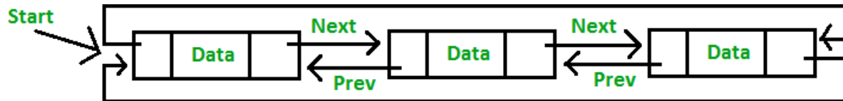
Circular Doubly Linked List
