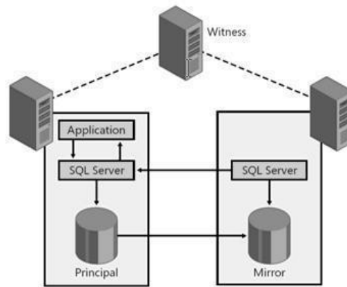
Gambar 1. Database Mirroring Architecture
