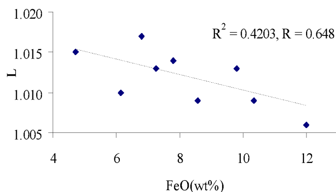
Figure. Plots of lineation (L) and FeO content showing negative correlation.
