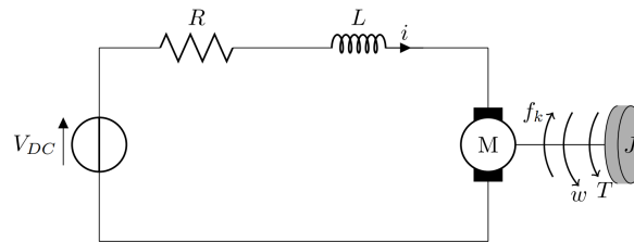
Gambar 1. Motor DC
