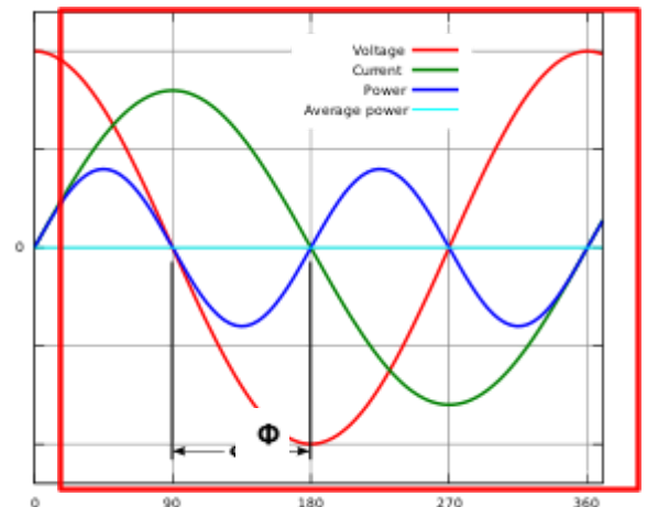
Figure 1.4 A Zero power factor
