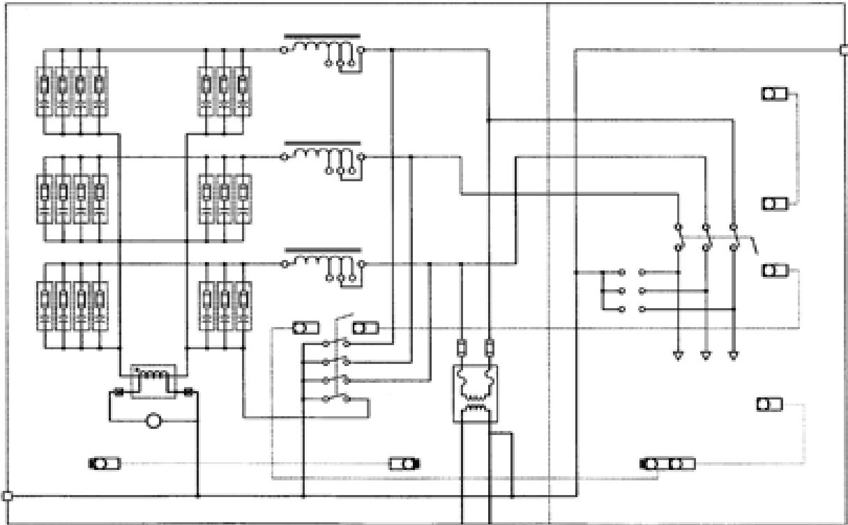
Figure 16.3 B: Harmonic Filter Banks installation
