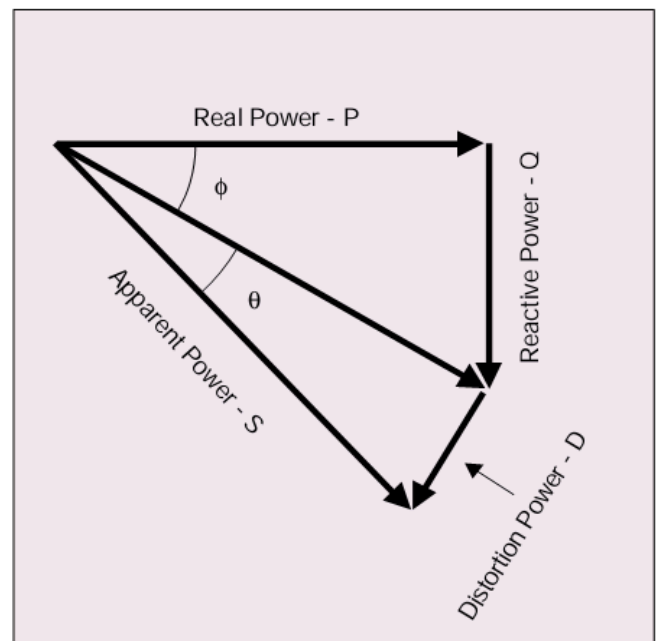
Figure 1.1: Power diagram of linear load
