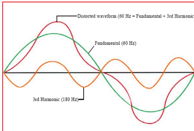
Figure 11: Harmonics wave form
