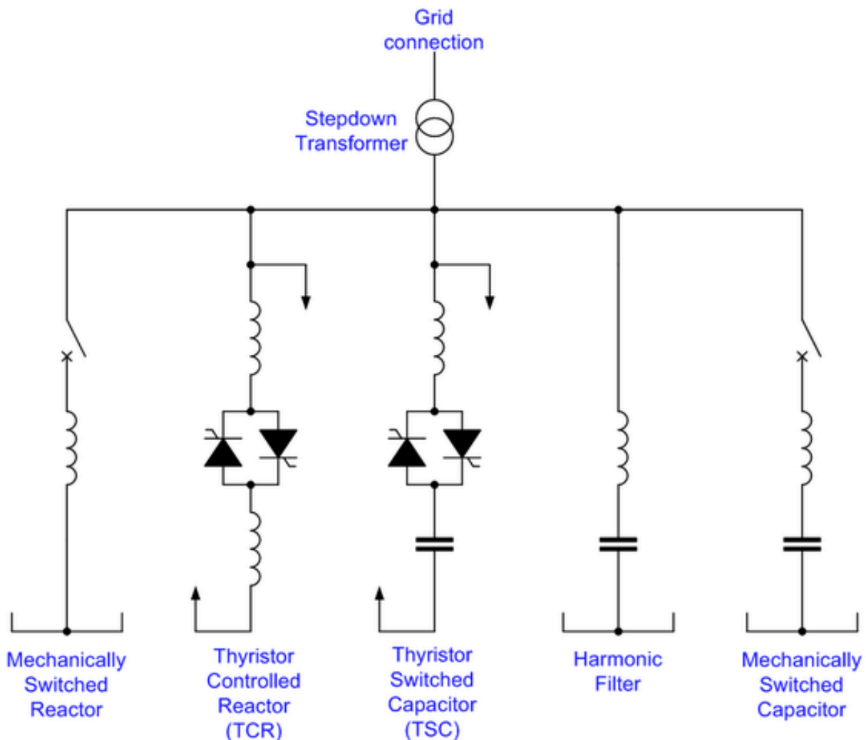
Figure 7.1B: SVC installation
