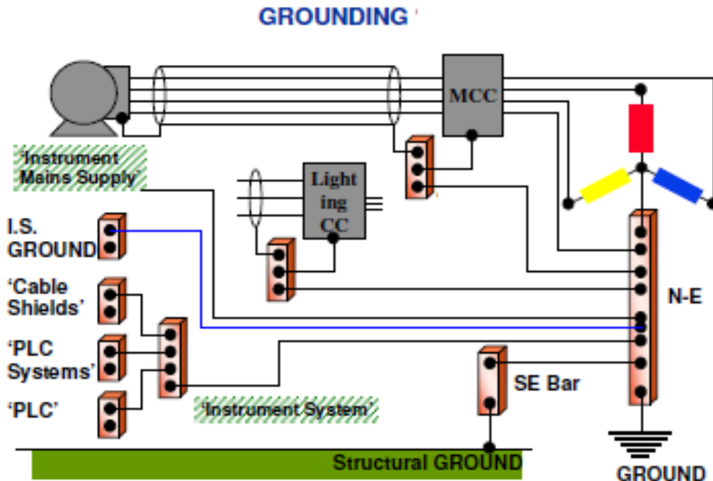
Figure 16.5: proper grounding
