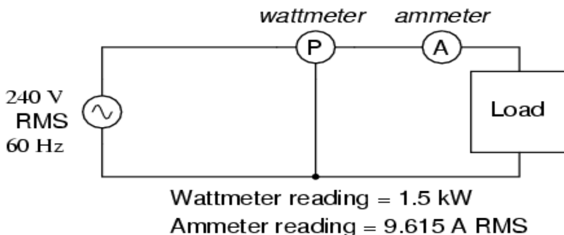
Figure 1.3: calculating PF by meters
