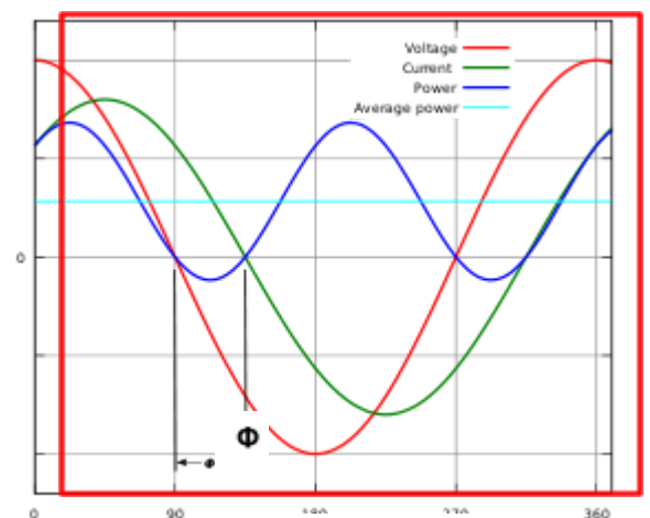
Figure 1.4 B Lagging power factor
