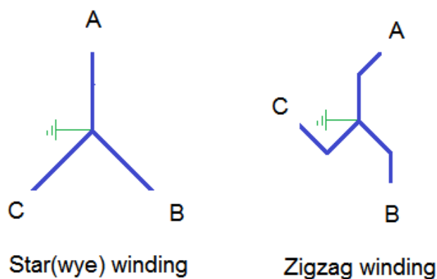
Figure 16.2 B: zig-zag winding
