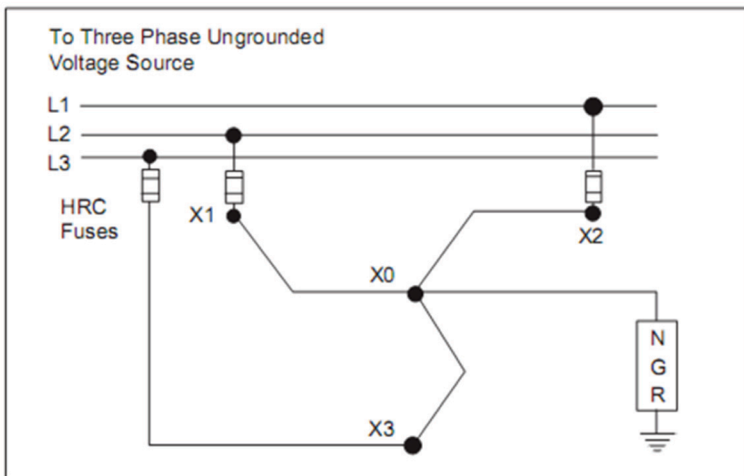
Figure 16.2 C: zig-zag transformer installation
