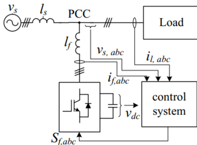
Figure 7.5: STATCOM installation
