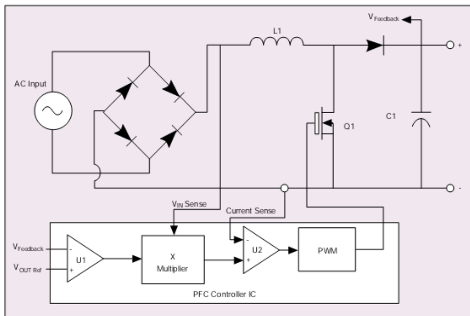
Figure 5.2 Boost circuit for active PFC: "High frequency"
