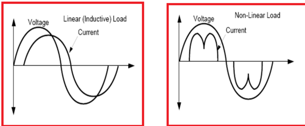
Figure 11.1 C: Linear Load vs. nonlinear load wave form
