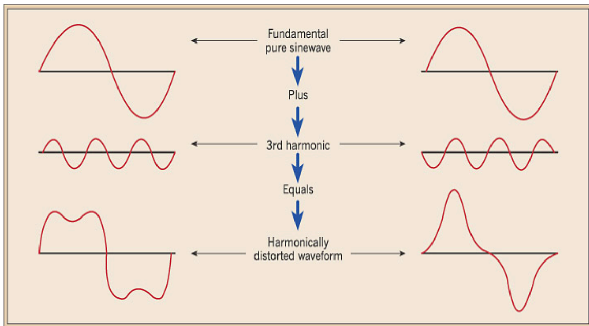
Figure 11.2: Harmonically distorted wave
