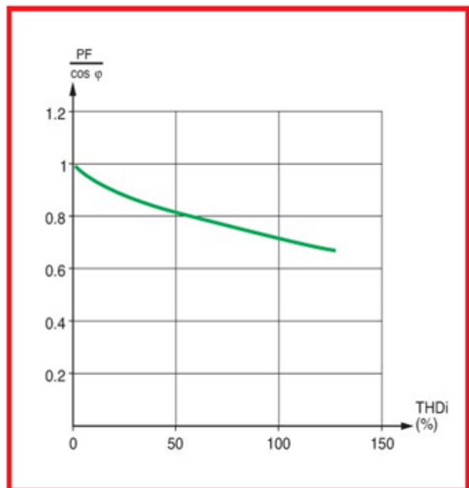
figure 13.1: graph of \frac{\text{PF}}{\cos\phi} as a function of THDi.
