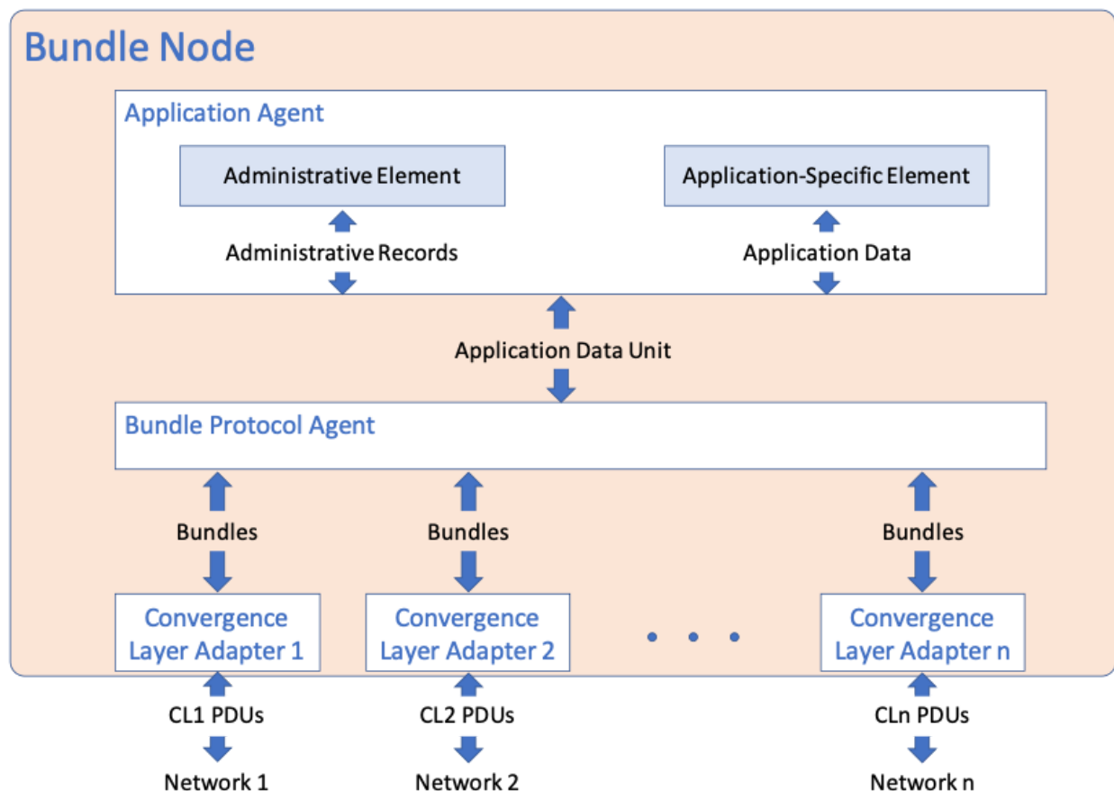
Figure 11-1 Graphical Representation of a Bundle Node": Graphical Representation of a Bundle Node
