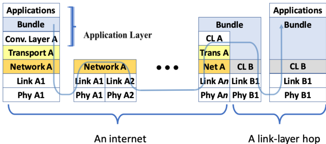
Figure 212-1 Bundle Protocol End-to-End Delivery Service": Bundle Protocol End-to-End Delivery Service
