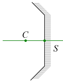
Miroir concave
