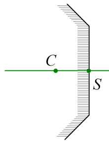
Miroir convexe
