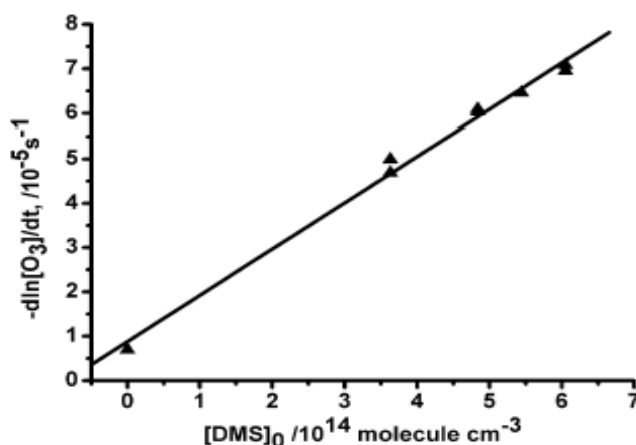
Fig. 2. Plot of -\frac{d \ln[O_3]}{dt} against [DMS]_0 .
