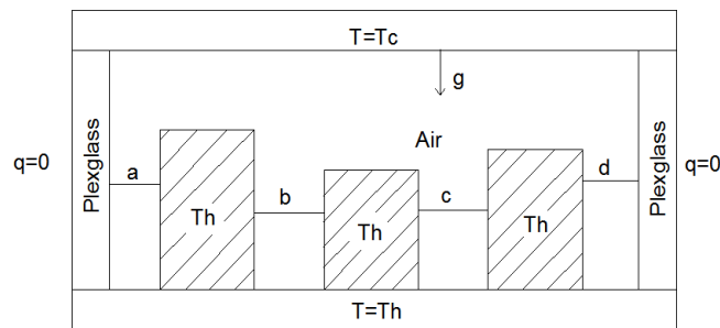
Gambar 1. Cavity geometry
