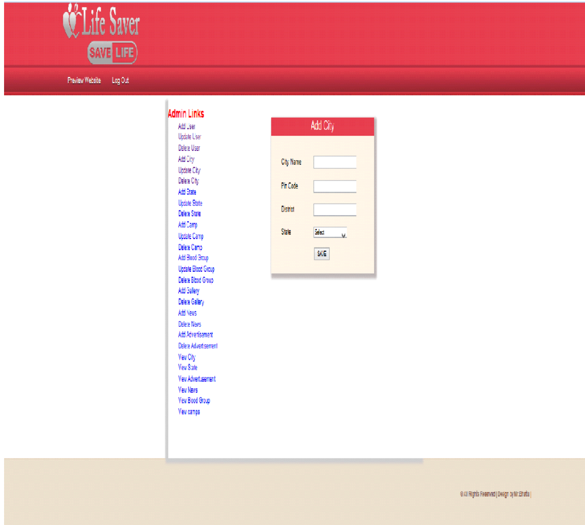
Figure 13.15: Add City
