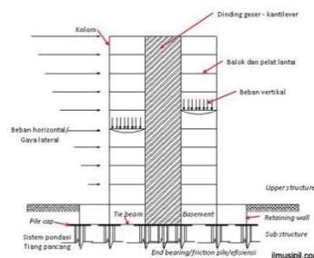
Figure 1. Loading on Multi-story Building
