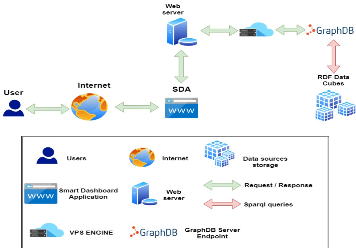
Figure 5.3: Allocation View
